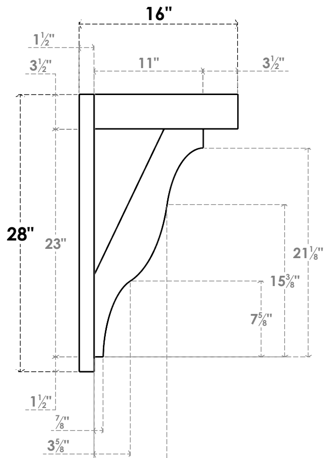
SIDE PROFILE
